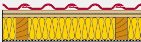
Pitched Roof with non-vapour permeable roofing system U-Value 0.17W/m²K
