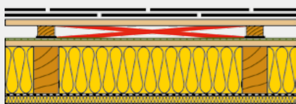
Pitched Roof with non-vapour permeable roofing system U-Value 0.14W/m²K
