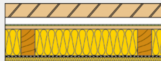
Timber Frame External Wall with service zone U-Value 0.15W/m²K
