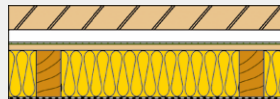
Timber Frame External Wall U-Value 0.19W/m²K
